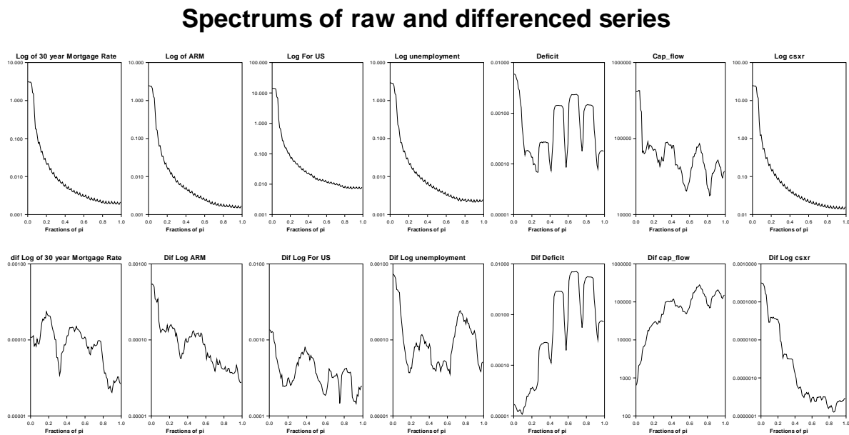
Figure 2. Spectrums of the raw and differenced series.
